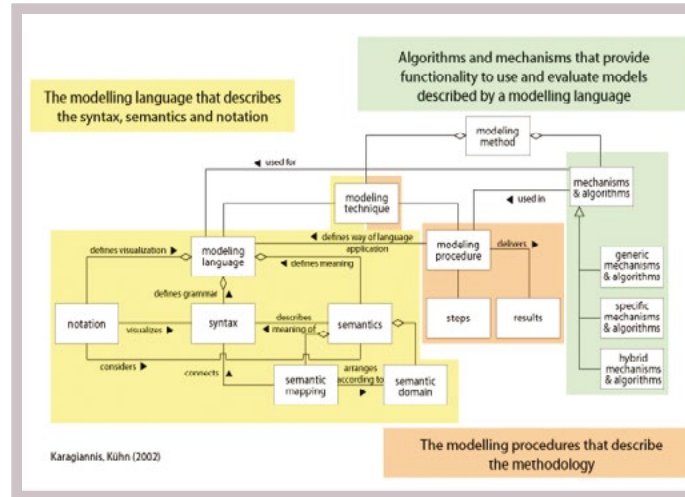
OMiLAB Modelling Method Engineering Framework
